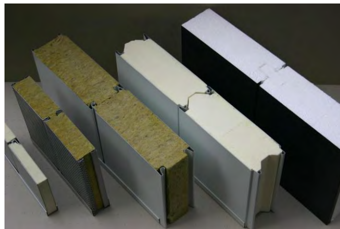
Selection of joints and core types
